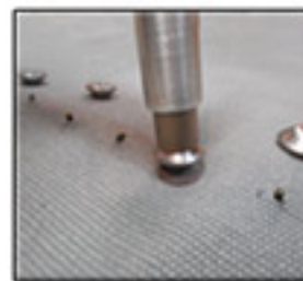
Using the tool, push the fastener down onto the cut shank
